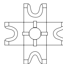
4-fold star blades for different cable diameters, V-radius blades in 3.49 / 4.37 / 6.20 / 7.70 mm
