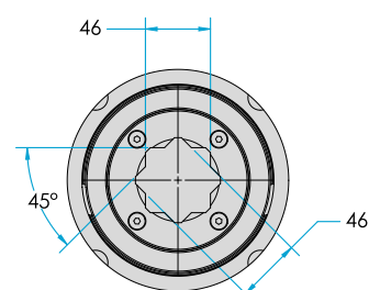
DETAIL F OPTIONAL ADAPTER ISO 5211 46mm SQUARE SHAFT INSERT MAX 4000Nm
