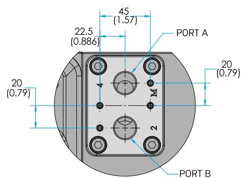
DETAIL H G-1/2" ISO FOR METRIC ACTUATOR 1/2" NPT FOR IMPERIAL ACTUATOR
